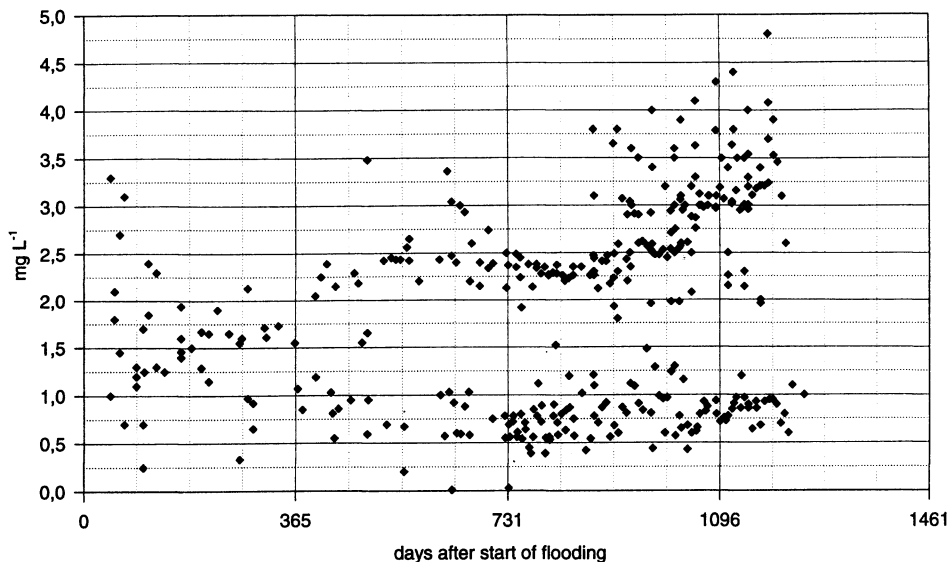
Fig. 3. Uranium mass concentration against time. Infiltration waters and flooding water can be distinguished by the content of U. 398 datapoints.
