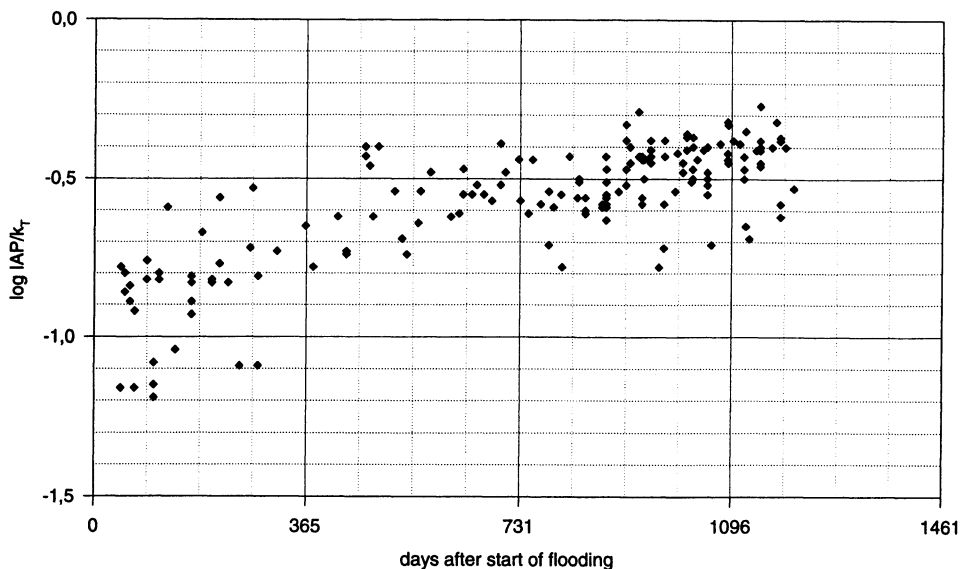
Fig. 4. Gypsum saturation index. Only results from flooding water analyses are plotted. 163 datapoints.
