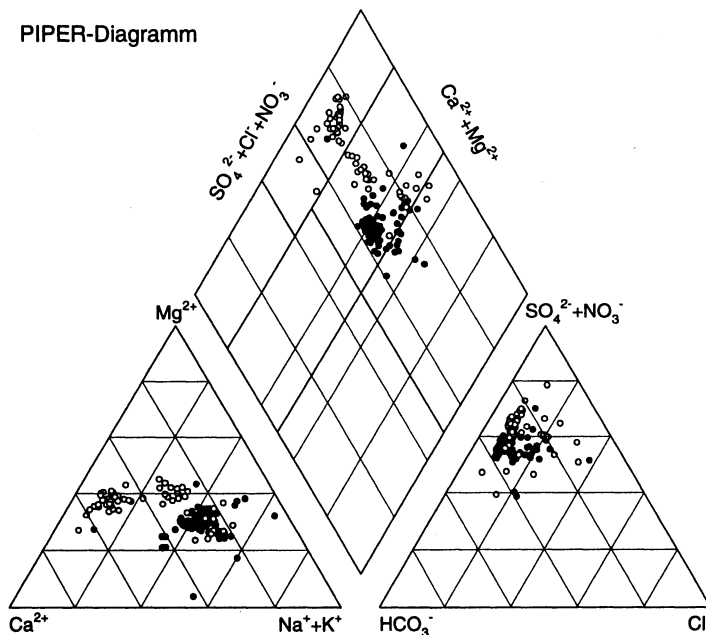
Fig. 2. Piper-diagram of 172 water samples from the Niederschlema/Alberoda U mine. Hollow circles: infiltration waters; closed circles: flooding water.
