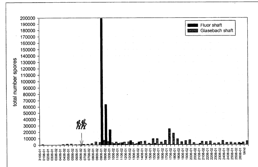
Fig. 3: Breakthrough diagram of the club moss spores detected at the Fluor and Glasebach shafts. Arrow marks time of tracer injection. No spores were detected at the No 539 shaft. Noticeable amounts of spores at the flour shaft arrive 2.5 days and at the Glasebach shaft 11 days after tracer injection.
