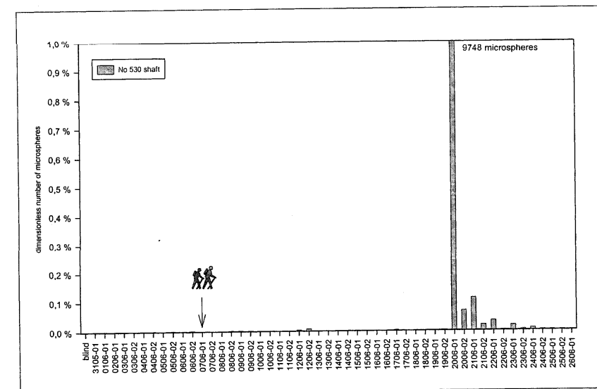
Fig. 5: Breakthrough diagram of the microspheres detected at the Glasebach shaft (max.: 9,748 microspheres). Arrow marks time of tracer injection.
