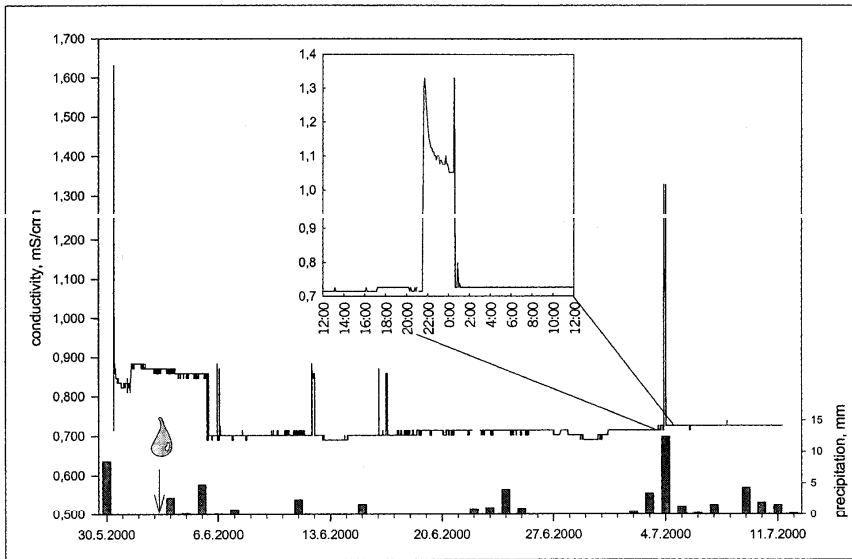
Fig. 2: Plot of precipitation (Siptenfelde station) and conductivity in the Fluor shaft. The arrow marks the time of the injection of the sodium chloride tracer into the Siptenfelde brook. Changes before June 6 th are due to moving the conductivity probe upwards in the shaft by 5 m.
